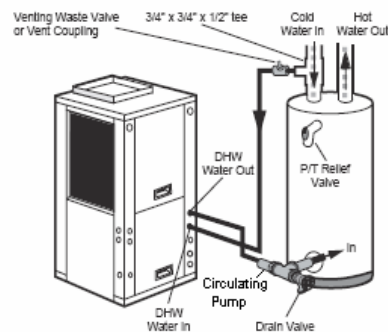
Figure 2: Typical Desuperheater Installation
