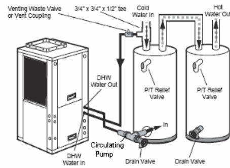
Figure 3: Desuperheater Installation In Preheat Tank
